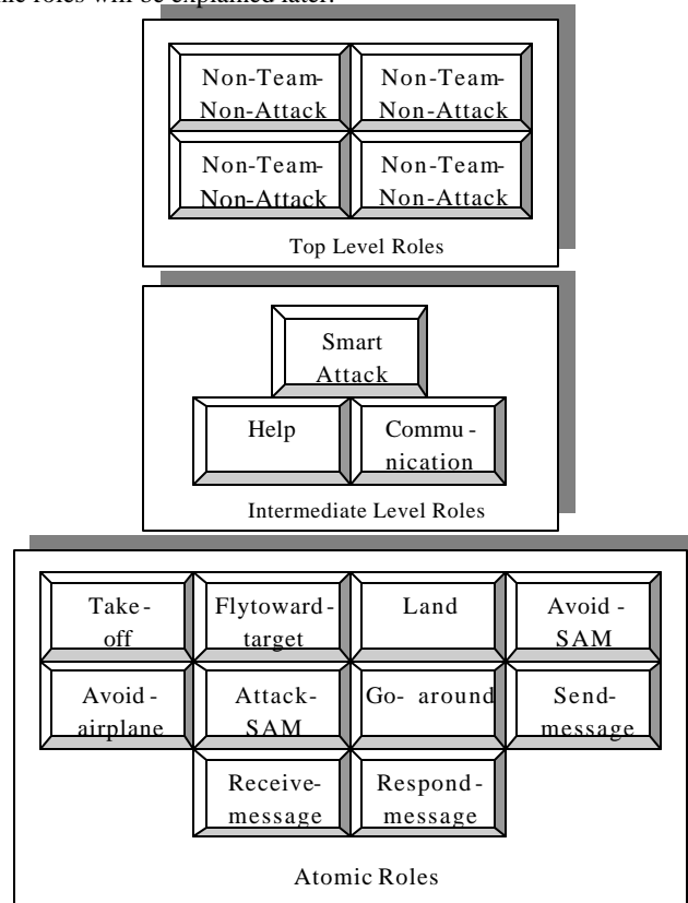
Figure 3 Role Hierarchy
