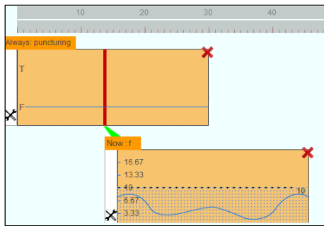
Fig. 6: The graphical formalism for \phi_{s1} .
