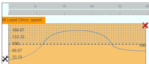
Fig. 2: Example 2: The graphical formalism for the Reachability MTL specification \phi_2 = \Diamond_{[0,39]}(\text{speed} > 100) .
