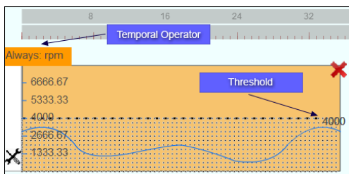
Fig. 1: Example 1: The graphical formalism for the Safety MTL specification \phi_1 = \Box_{[0,36]}(\text{rpm} < 4000) .
