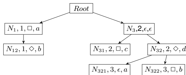
Fig. 4: The corresponding tree structure for formula \phi = \Box(a \wedge \Diamond b) \rightarrow (\Box c \wedge \Diamond(d \rightarrow (a \wedge \Box b))) where a, b, c and d are predicates. Each node is composed of a node name, group number, temporal operator, and predicate. The symbol \epsilon indicates empty parameters.
